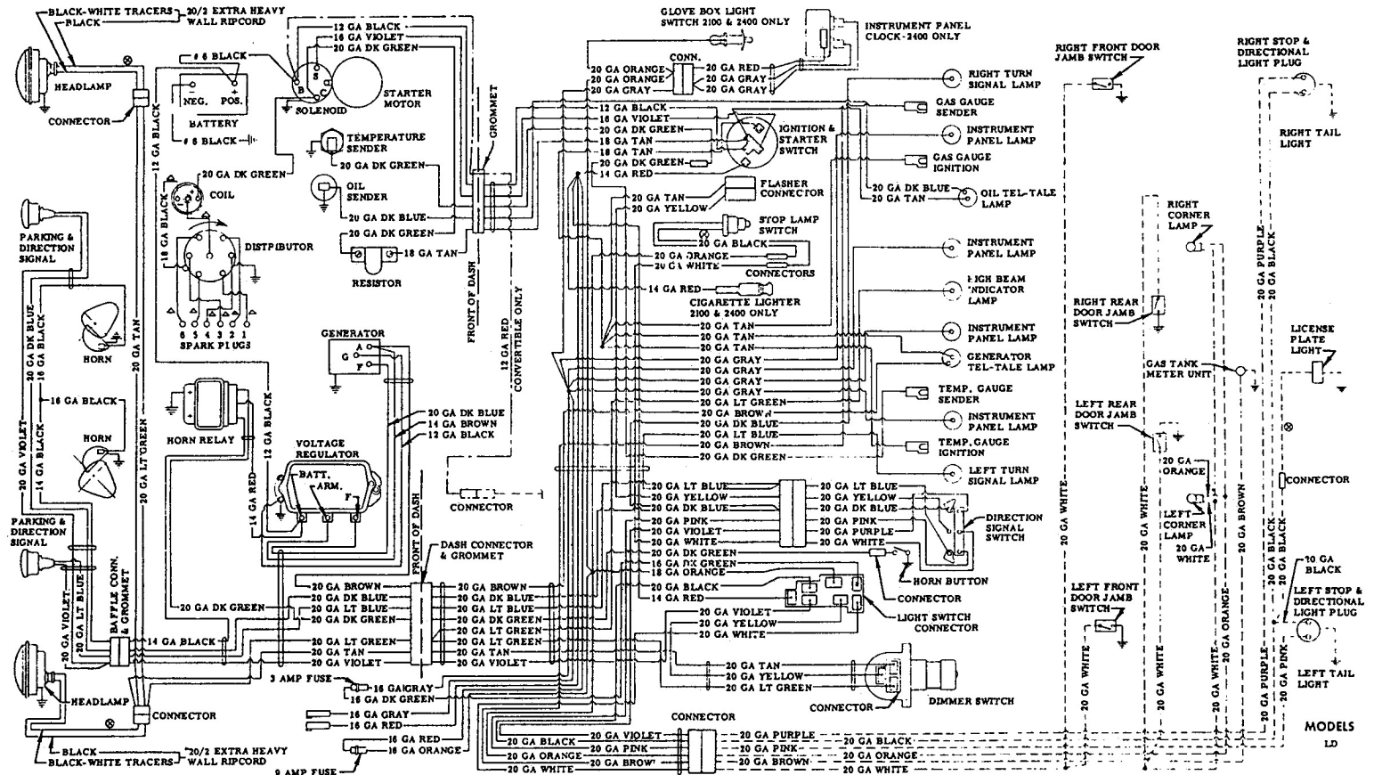
WIRING DIAGRAM
