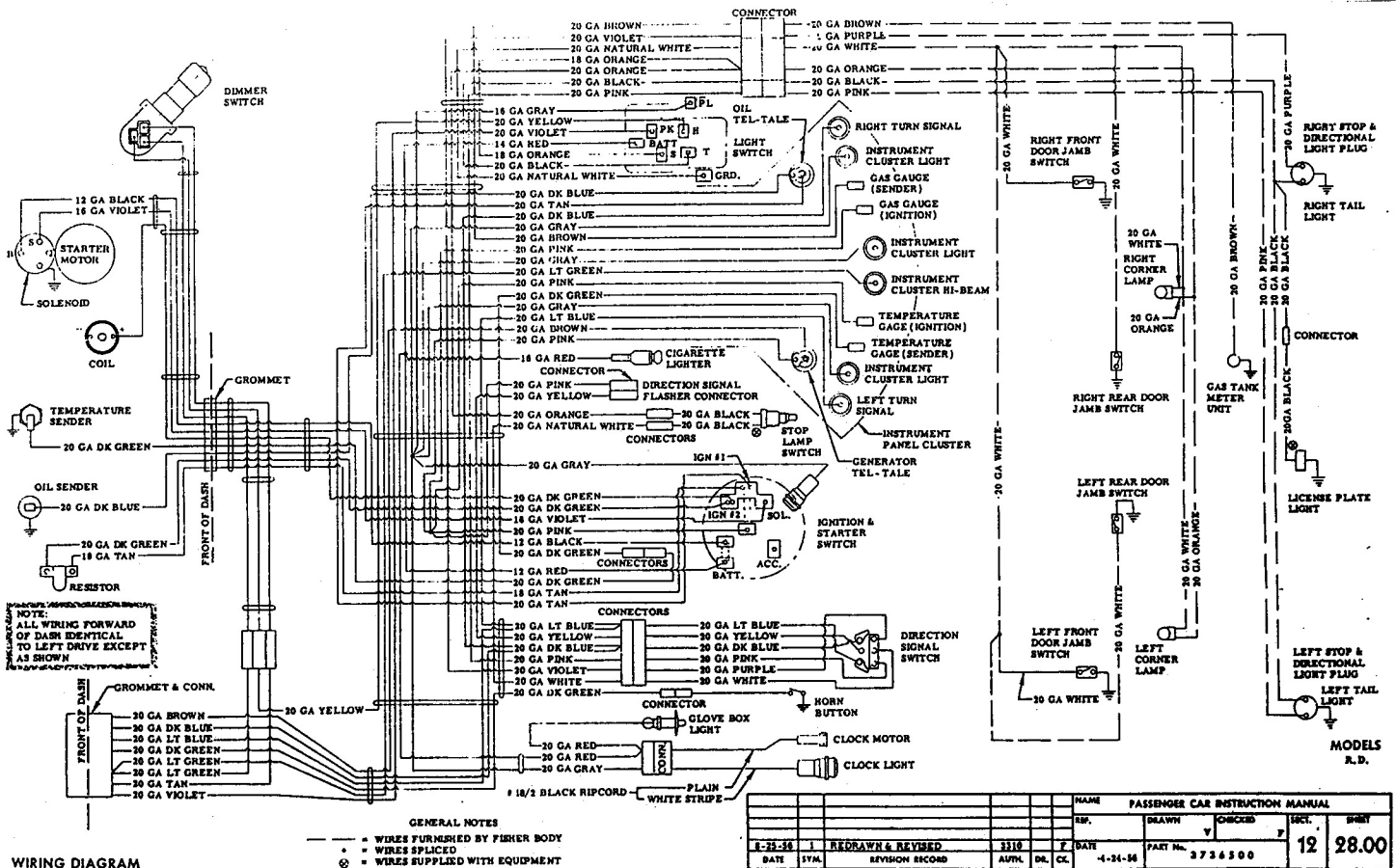
WIRING DIAGRAM
